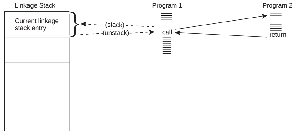
Figure 6-7. Two Programs Sharing a SCOPE=SINGLE Data Space
