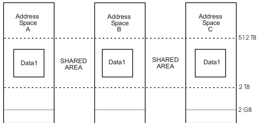
Figure 4-3. z/OS R5 Address Space with the default shared area between 2-terabytes and 512-terabytes
