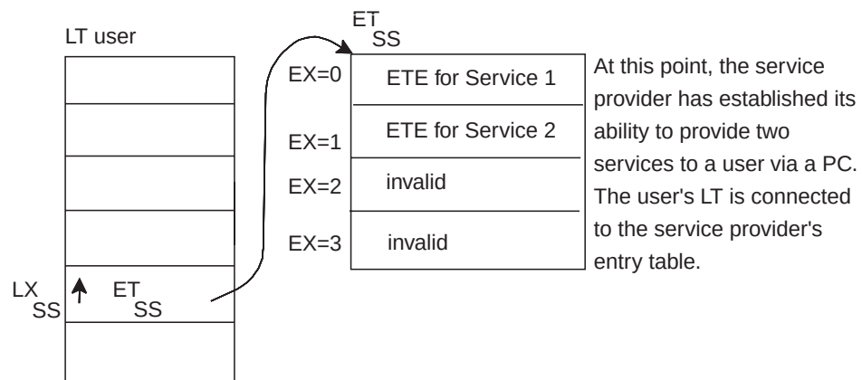
Figure 3-10. Linkage Table and Entry Table Connection
