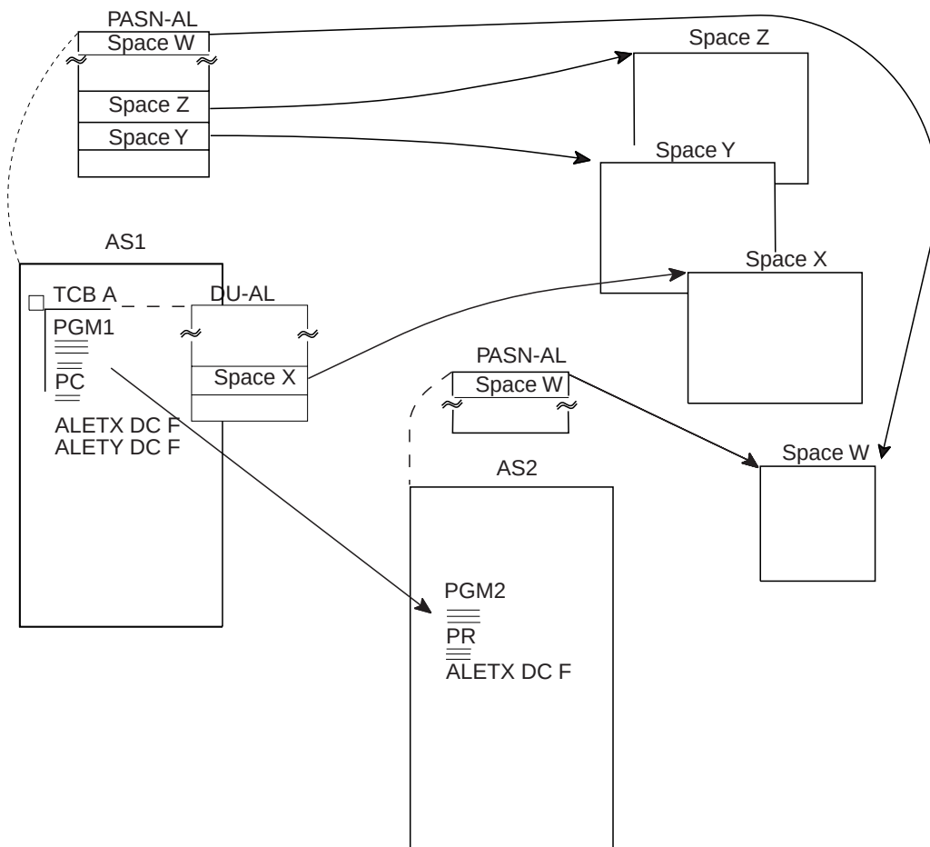
Figure 5-6. PASN-ALs and DU-ALs at a Space Switch
