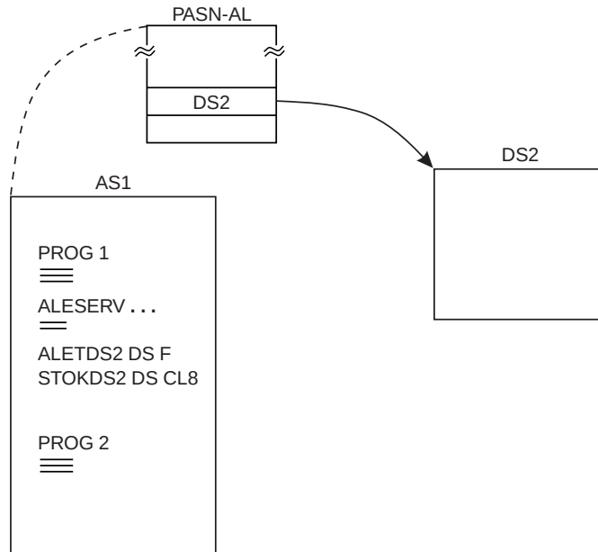
Figure 5-10. Example 2: Adding an Entry to a PASN-AL
