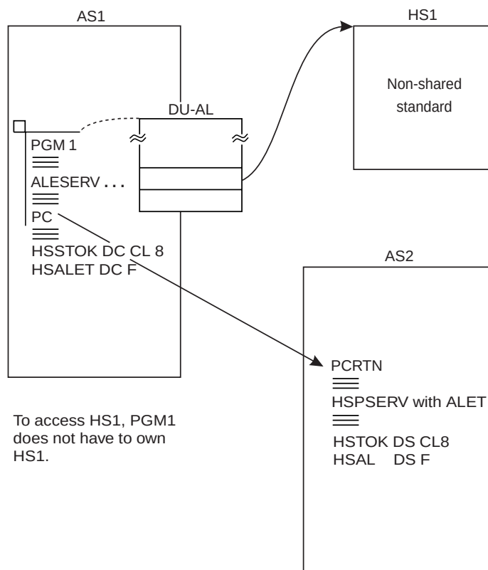
Figure 7-6. Example 2: An Unauthorized Program Using a Standard Hiperspace
