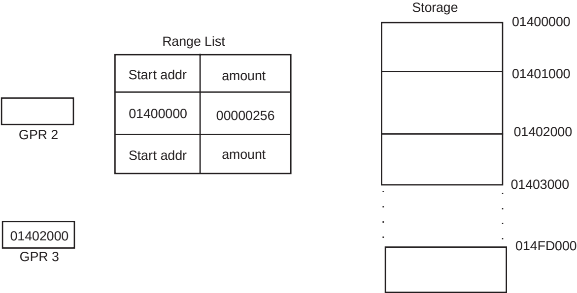
Figure 9-4. Illustration of GPR Contents in Event of Range List Error
