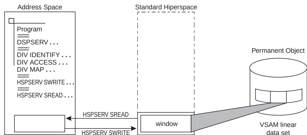
Figure 7-13. Example of Mapping a Data-in-Virtual Object to a Hiperspace
