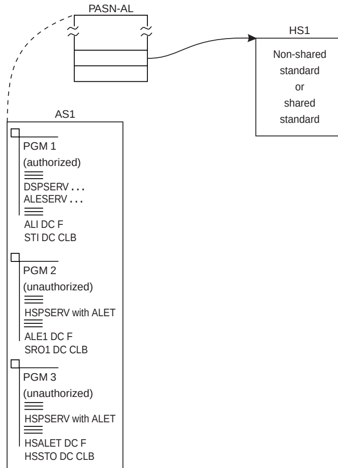
Figure 7-5. Example 1: An Unauthorized Program Using a Standard Hiperspace
