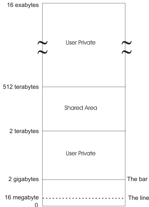
Figure 4-1. z/OS R5 Address Space
