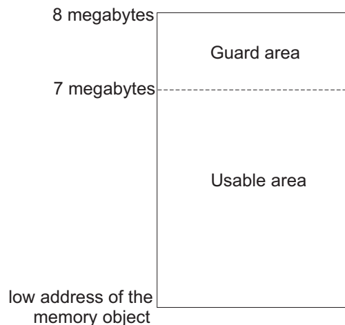
Figure 4-4. A memory object eight megabytes in size
