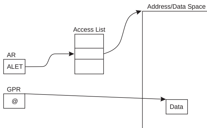
Figure 5-2. Using an ALET to Identify an Address/Data Space
