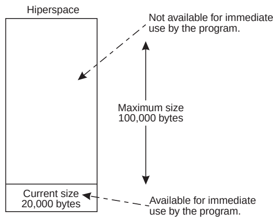
Figure 7-2. Example of Specifying the Size of a Hiperspace
