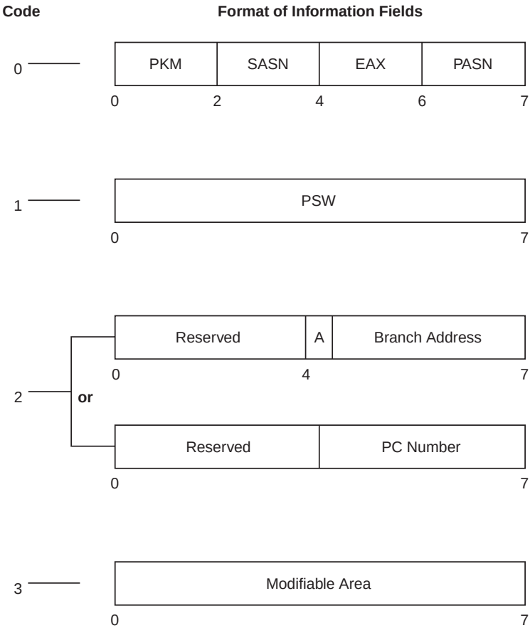
Figure 2-4. Format of the Information Fields
