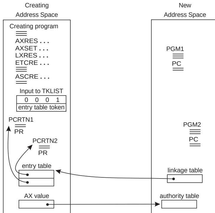
Figure 8-4. The Cross Memory Linkages Set by the ASCRE Macro
