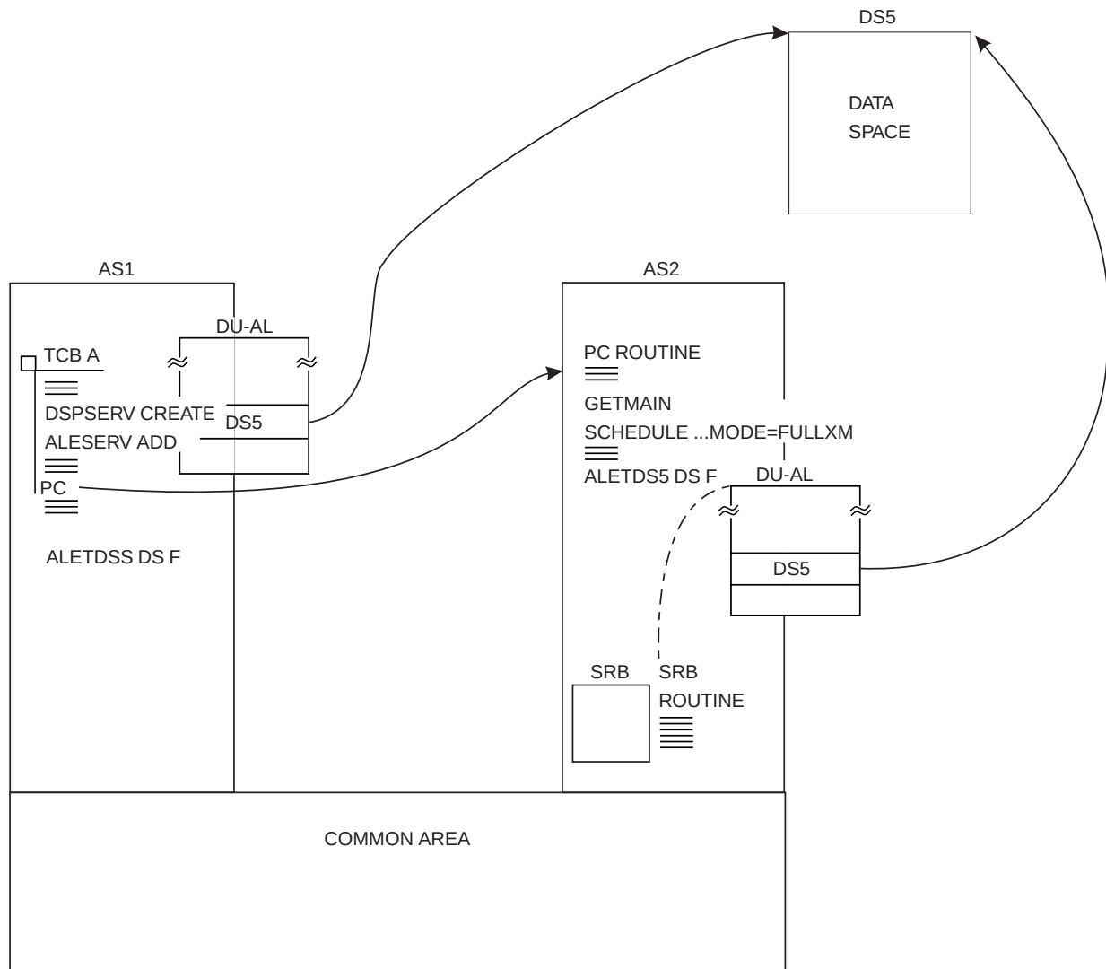
Figure 6-10. Scheduling an SRB with a Copy of the Scheduling Program's DU-AL and in the Same Cross Memory Environment
