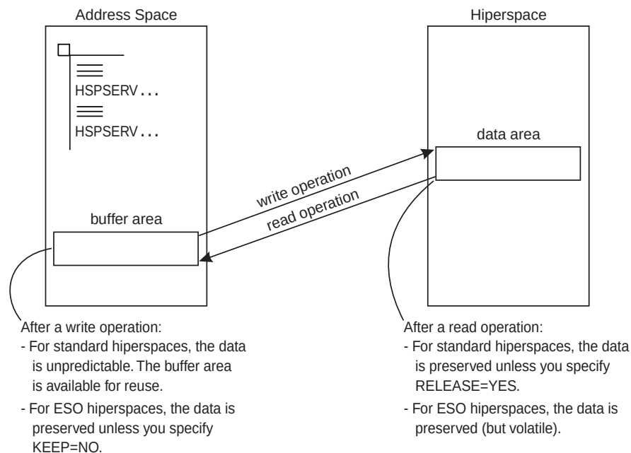
Figure 7-9. Illustration of the HSPSERV Write and Read Operations
