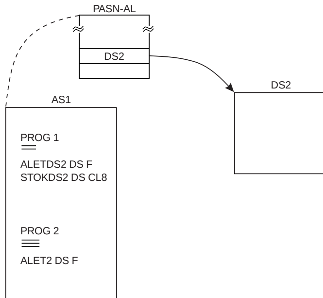
Figure 5-11. Example 2: Sharing a Data Space through the PASN-AL
