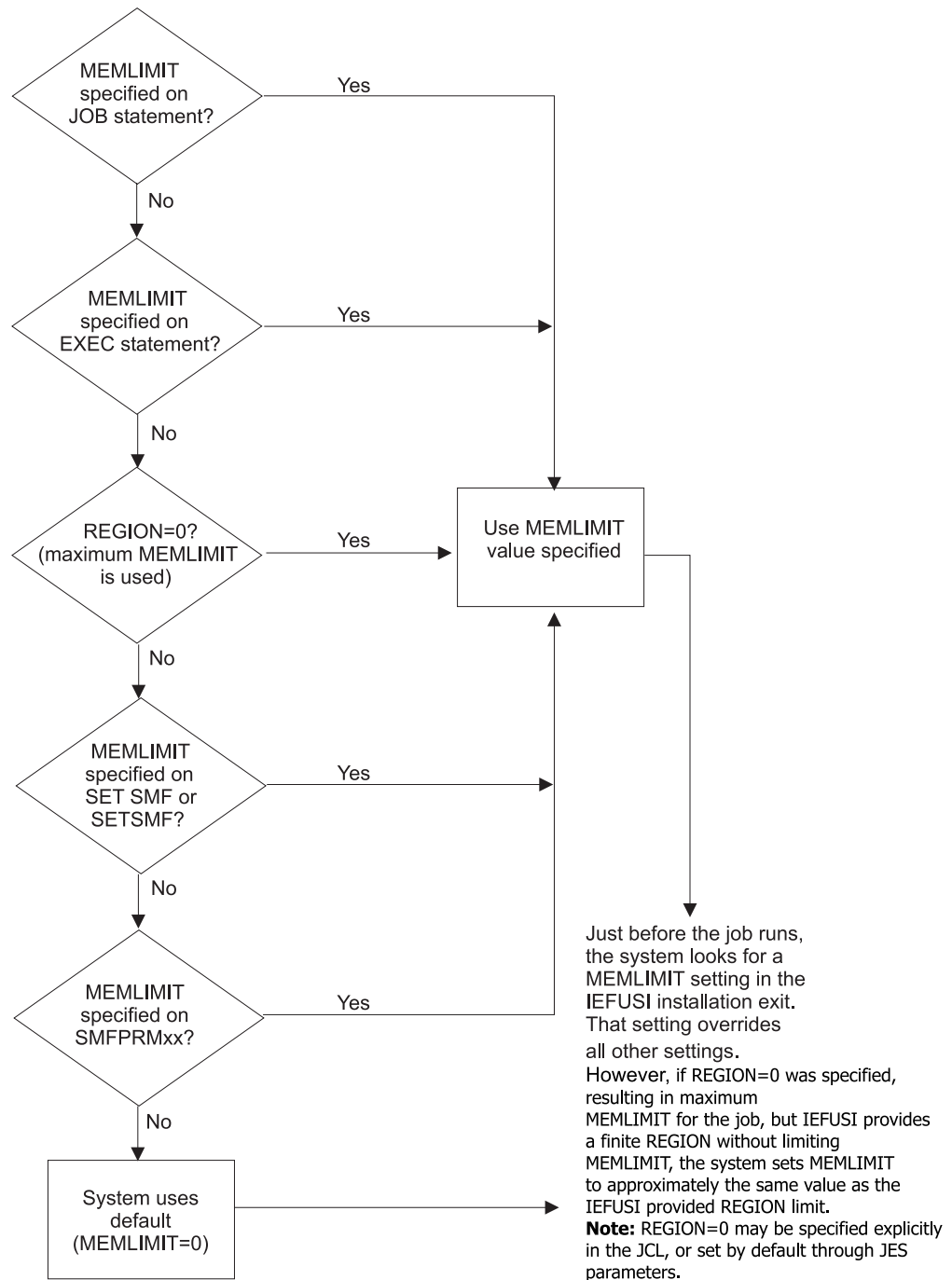
Figure 4-2. How the System Chooses which MEMLIMIT Applies
