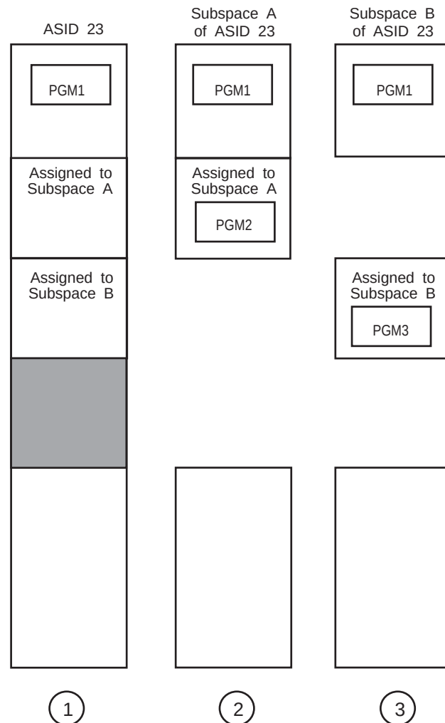
Figure 9-2. Illustration of Address Space that Owns Two Subspaces
