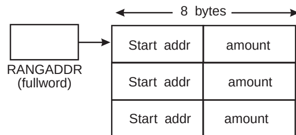
Figure 9-3. Illustration of the Range List
