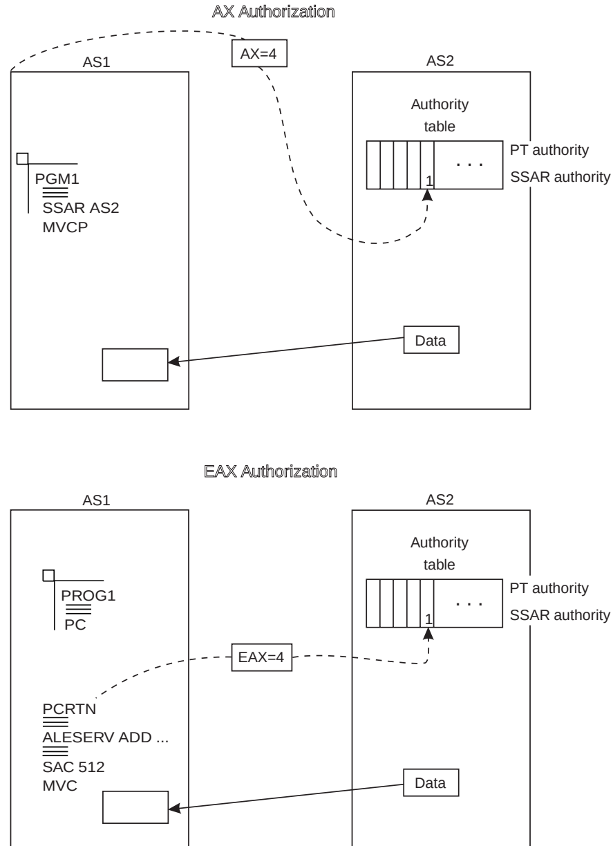
Figure 5-16. Comparison of an AX and an EAX
