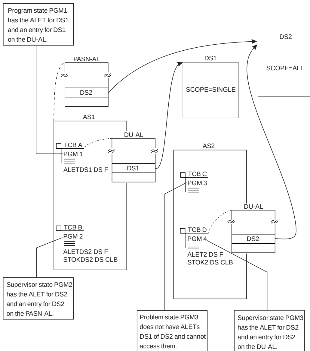
Figure 6-1. Example of Rules for Accessing Data Spaces
