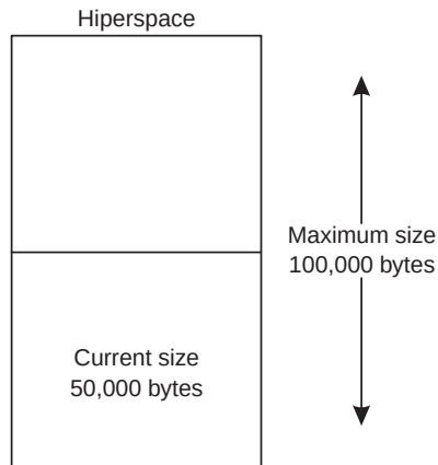
Figure 7-12. Example of Extending the Current Size of a Hiperspace
