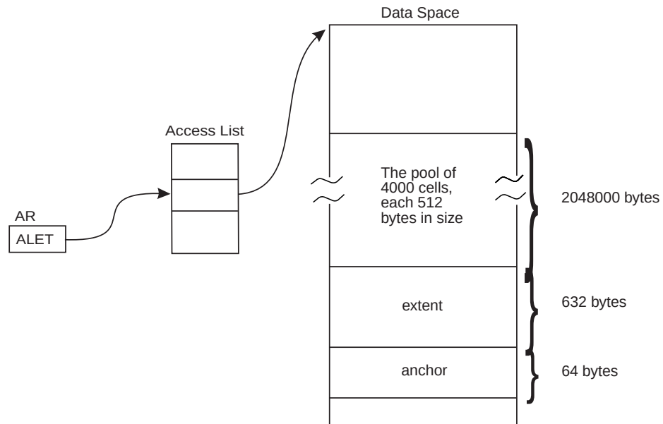
Figure 6-4. Example of Using Callable Cell Pool Services for Data Spaces
