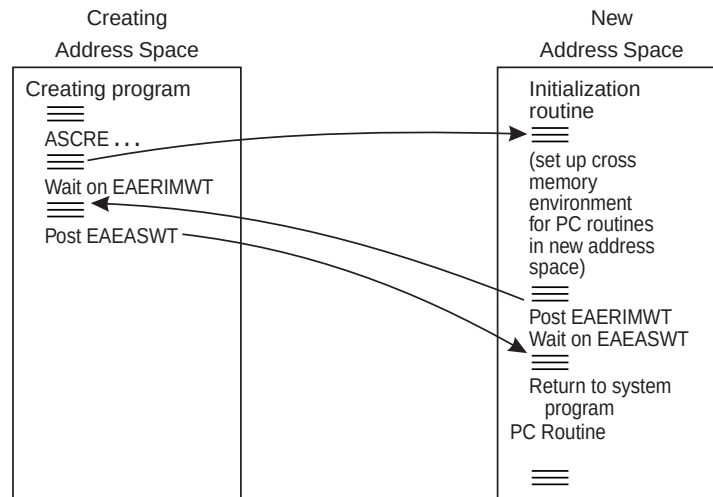
Figure 8-1. Synchronization of the Address Space Creation Process
