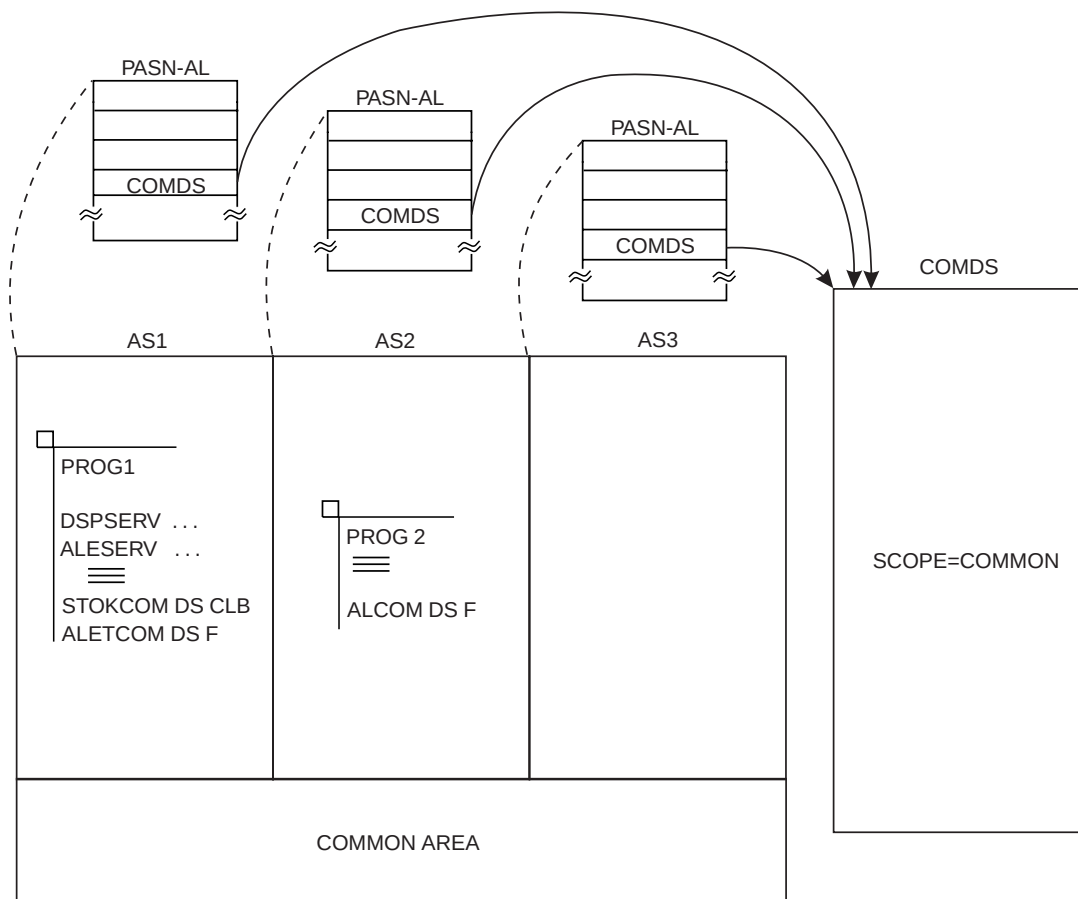
Figure 6-6. Example of Using a SCOPE=COMMON Data Space
