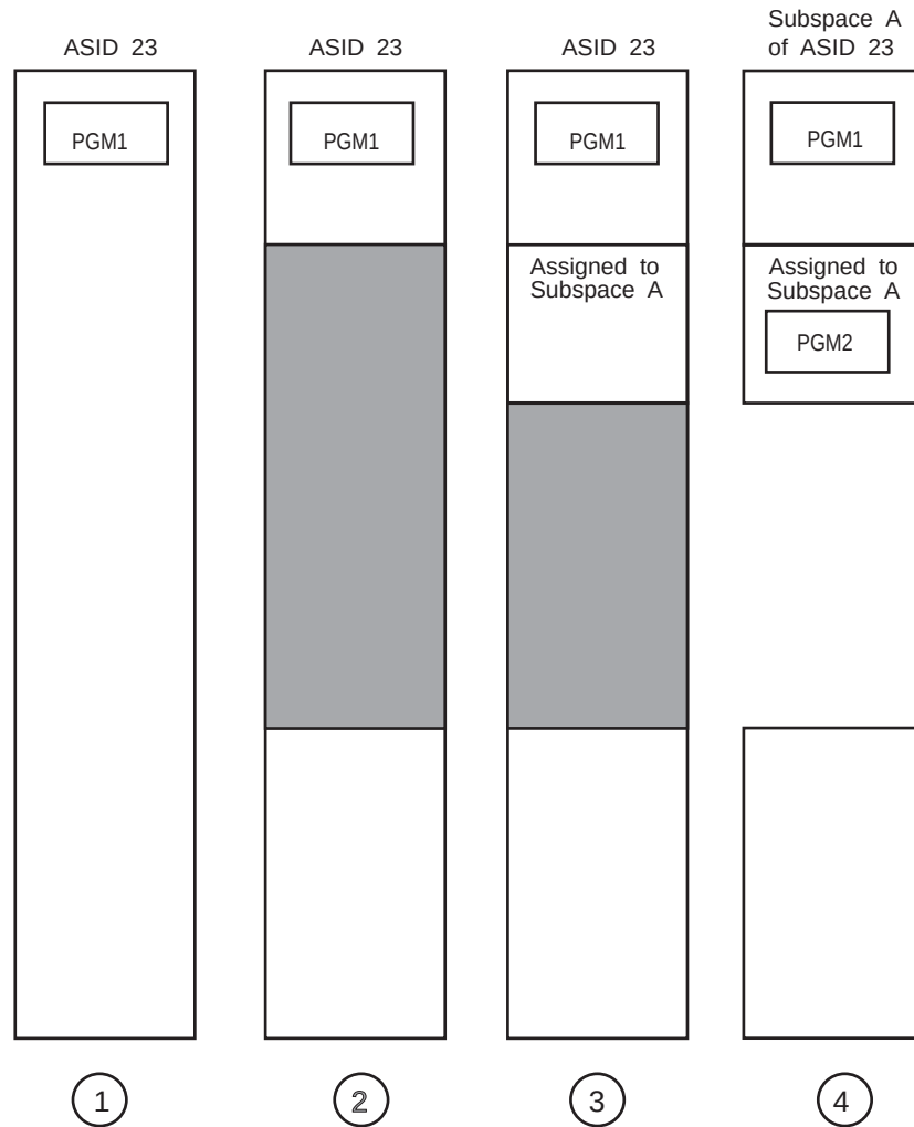
Figure 9-1. Illustration of Address Space that Owns One Subspace
