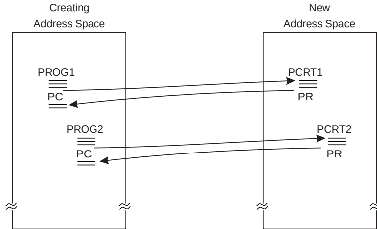
Figure 8-2. An Example of a Cross Memory Environment
