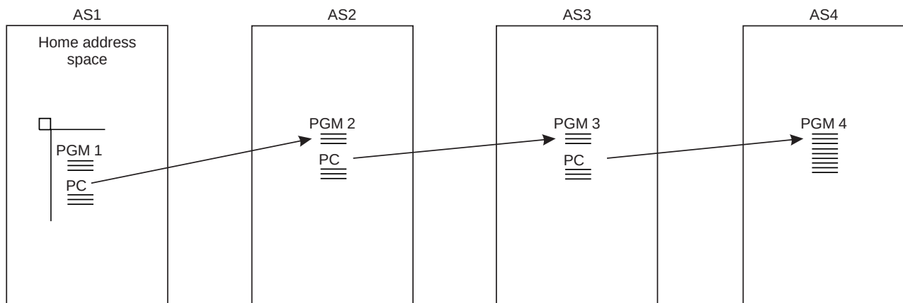
Figure 5-14. Using the ALET for the Home Address Space
