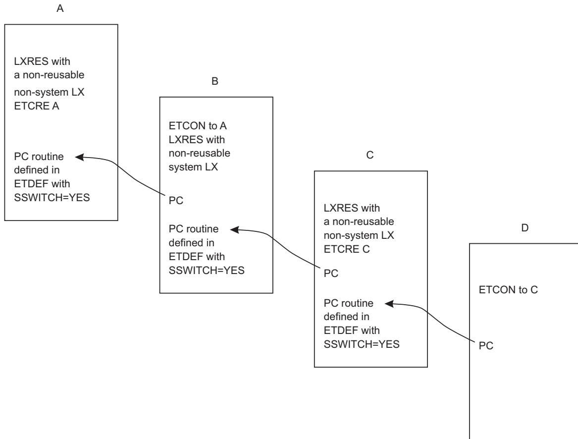
Figure 3-15. Cross Memory Connections between Address Spaces
