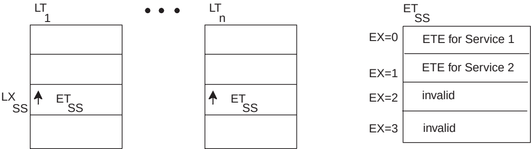
Figure 3-13. Linkage and Entry Tables for a Global Service
