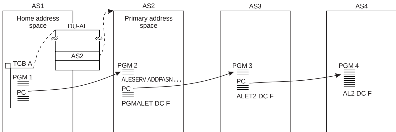
Figure 5-13. Obtaining the ALET for the Primary Address Space
