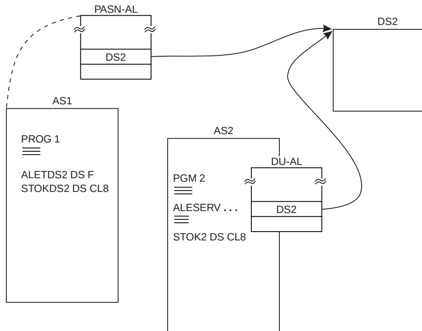
Figure 5-12. Example 3: Sharing Data Spaces Between Two Address Spaces
