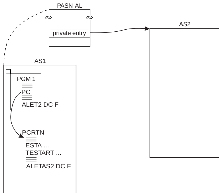
Figure 5-17. Checking the Validity of an ALET
