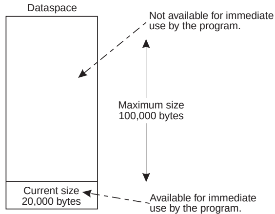
Figure 6-2. Example of Specifying the Size of a Data Space
