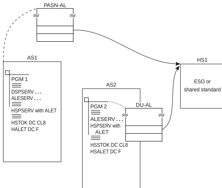
Figure 7-11. Gaining Fast Data Transfer To and From Expanded Storage
