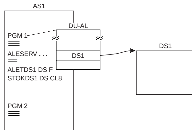
Figure 5-8. Example 1: Adding an Entry to a DU-AL
