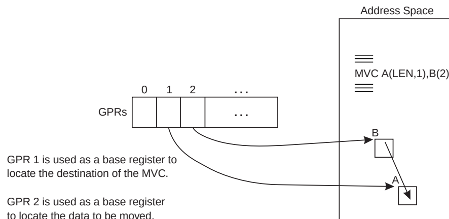
Figure 5-3. The MVC Instruction in Primary Mode
