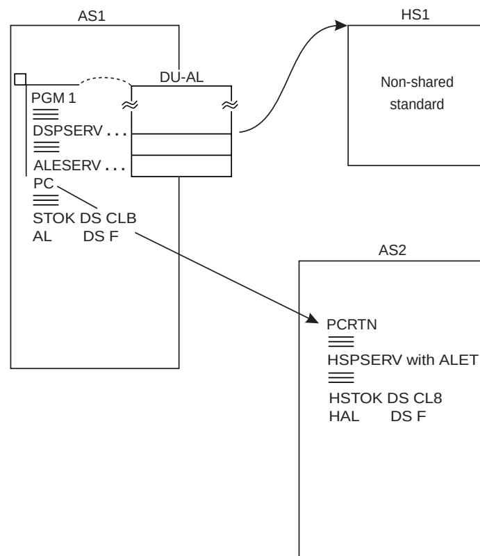
Figure 7-7. A Supervisor State Program Using a Non-Shared Standard Hiperspace
