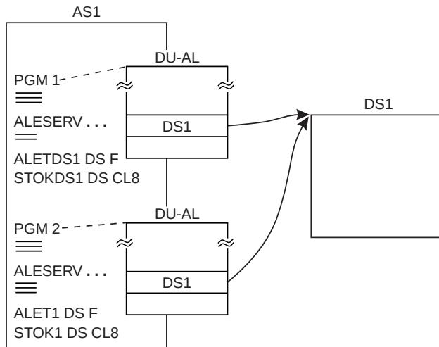
Figure 5-9. Example 1: Sharing a Data Space through DU-ALs
