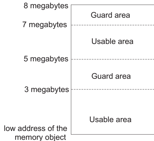
Figure 4-5. A memory object with an additional guard area
