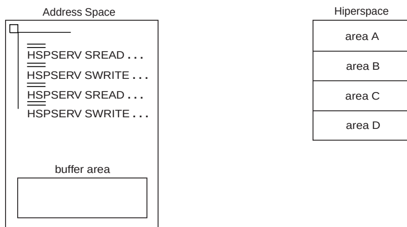
Figure 7-1. Example of Scrolling through a Standard Hiperspace
