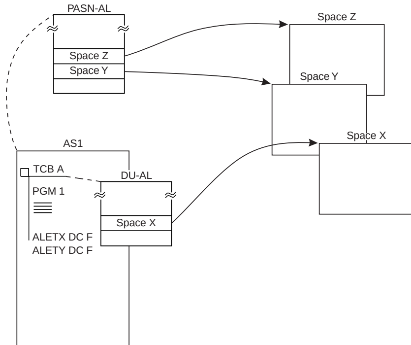
Figure 5-5. Comparison of Addressability through a PASN-AL and a DU-AL
