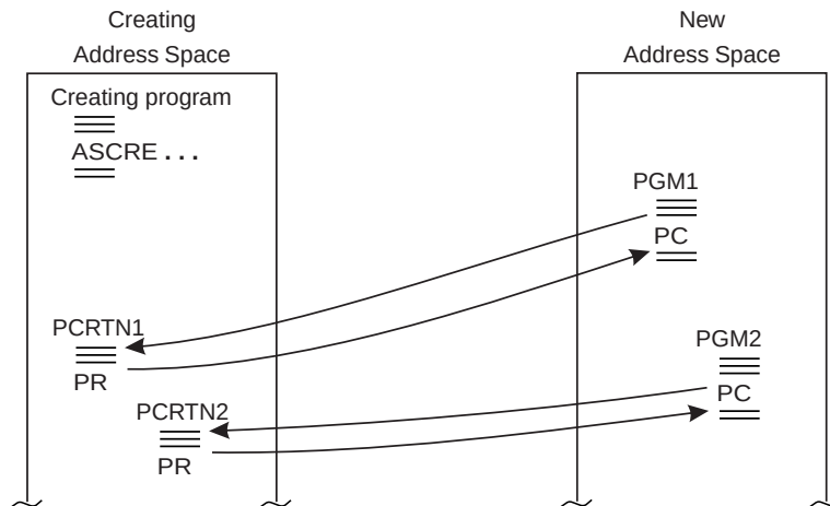
Figure 8-3. An Example of Cross Memory Environment Set by the ASCRE Macro
