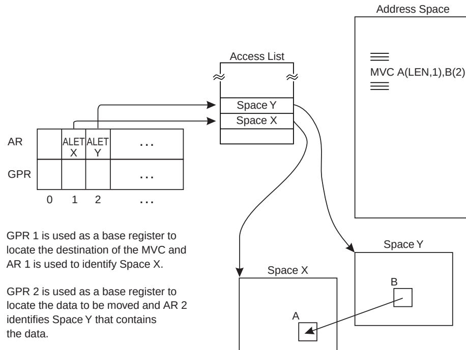
Figure 5-4. The MVC Instruction in AR Mode
