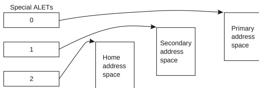
Figure 5-7. Special ALET Values
