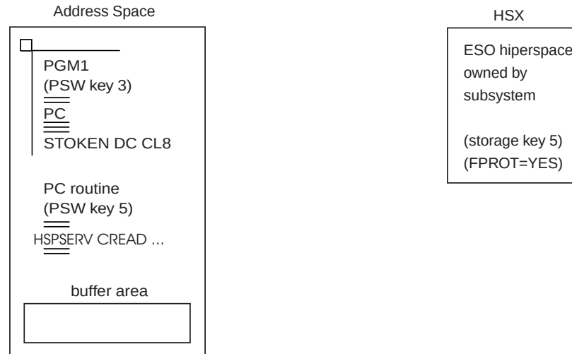
Figure 7-3. Protecting Storage in a Hiperspace
