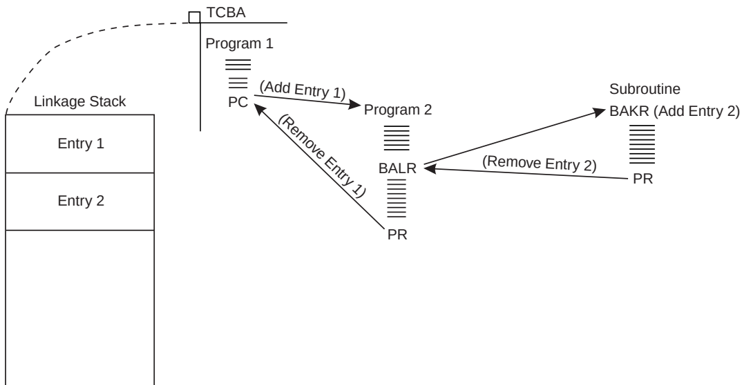
Figure 2-2. Example of Using the Linkage Stack
