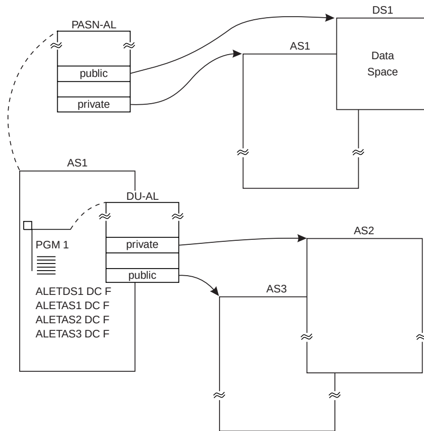
Figure 5-15. Difference Between Public and Private Entries
