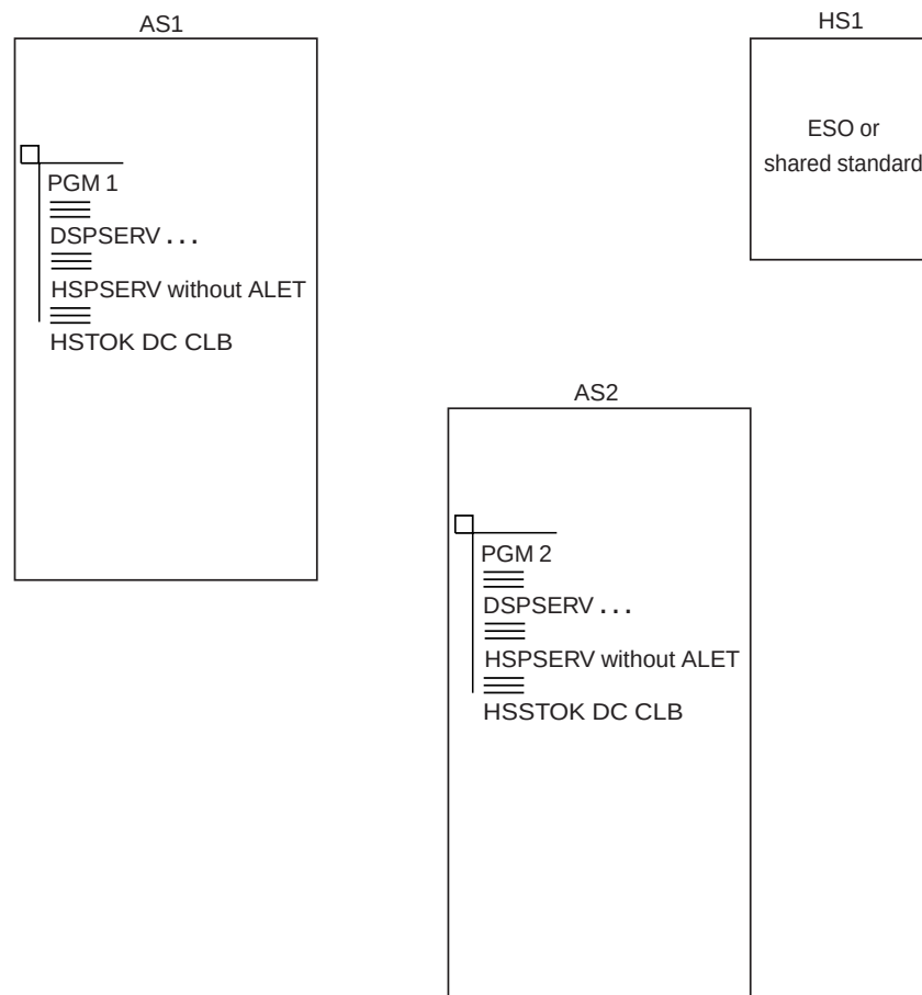
Figure 7-8. A Supervisor State Program Using a Shared Standard Hyperspace
