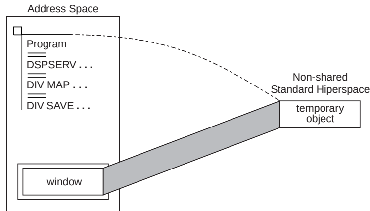
Figure 7-14. A Standard Hiperspace as a Data-in-Virtual Object
