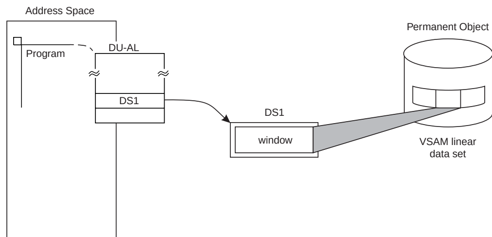
Figure 6-8. Example of Mapping a Data-in-Virtual Object to a Data Space
