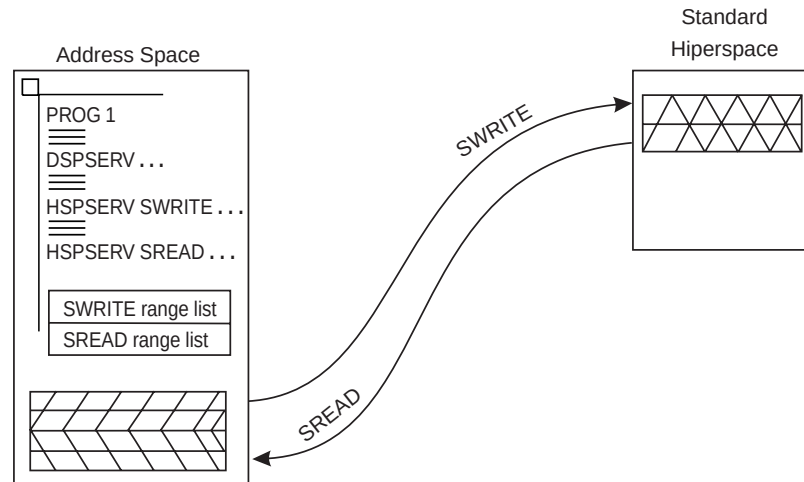
Figure 7-10. Example of Creating a Standard Hiperspace and Transferring Data
