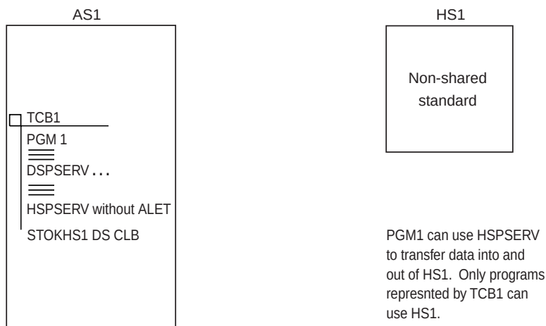
Figure 7-4. A Problem State Program Using a Non-shared Standard Hiperspace
